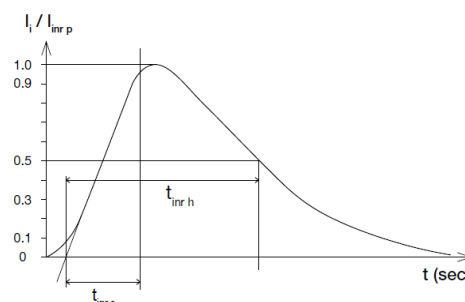
Figure 6. Inrush Current
