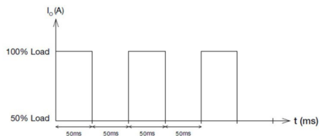
Figure 5. Dynamic Load
